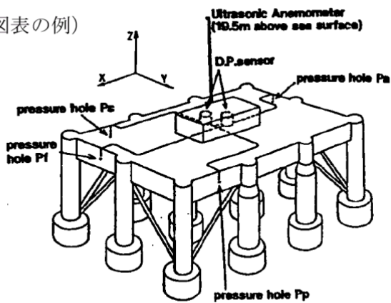
Fig. 16 Measurement of wind pressures
